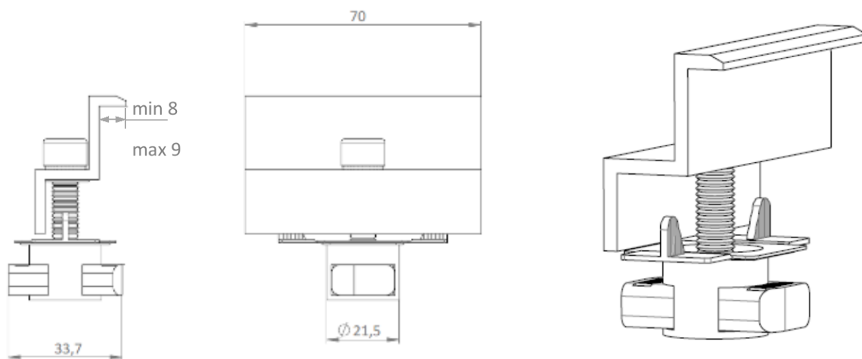
Figure 13 : Étrier final
