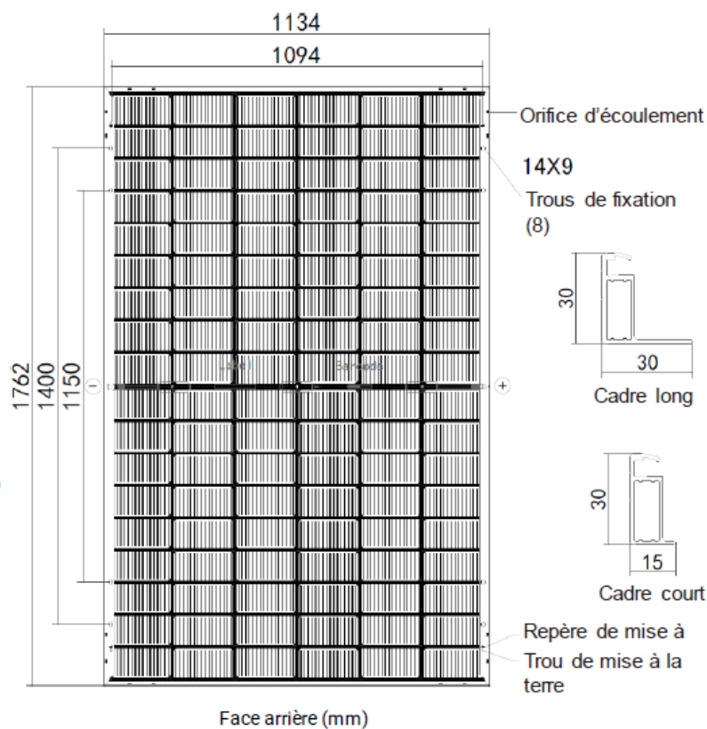
Modules DMxxxM10RT-B54HSW/HBW/HBT
