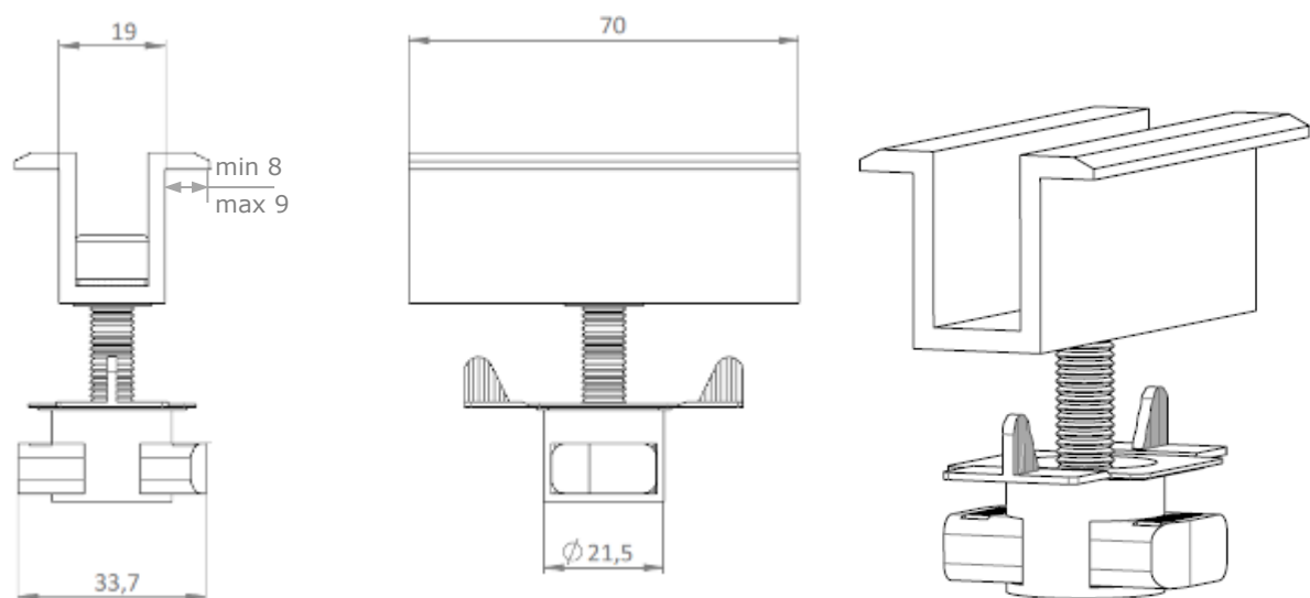
Figure 12 : Étrier final
